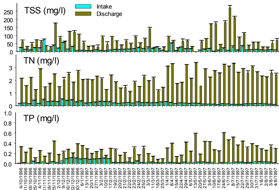
Figure 8. Intake and discharge nutrient concentrations, Seafarm, 1996/97.
