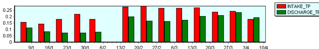
Figure 32. Total Phosphorus (TP) concentration, mg.L -1 , in treatment pond intake and discharge water, GCMPPF, 1999.
