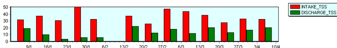
Figure 30. Total Suspended Solids (TSS) concentration, mg.L -1 , in treatment pond intake and discharge water, GCMPPF, 1999.
