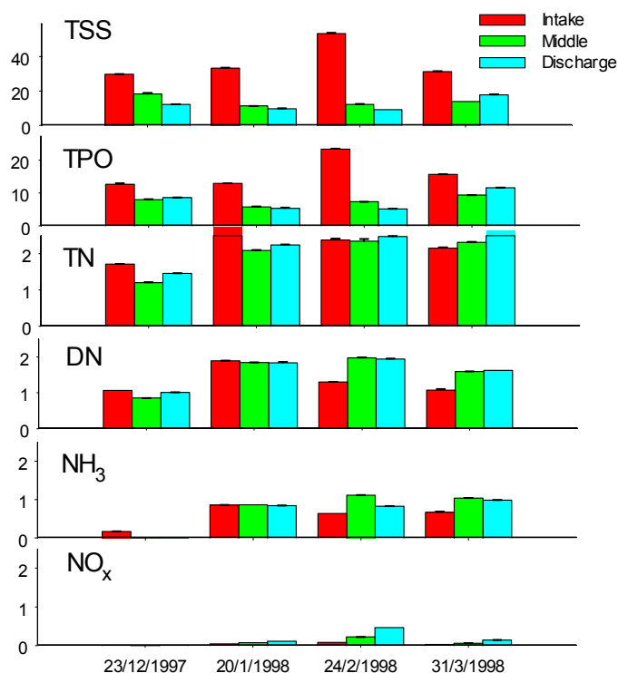
Figure 28. Changes in water quality in GCMFP treatment pond during the 1997/98 season – all results in mg.L -1 . See Figure 7, Methods, for sampling locations. TSS, total suspended solids; TPO, total particulate organics; TN, total nitrogen; DN, dissolved nitrogen; NH 3 , total ammonia nitrogen; NO x , nitrogen oxides (NO 3 + NO 2 ).
