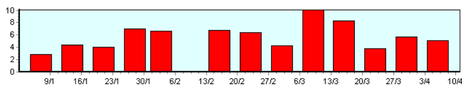
Figure 35. Total Nitrogen (TN) removal (kg.ha -1 .d -1 ), GCMPPF pilot treatment pond, 1999.
