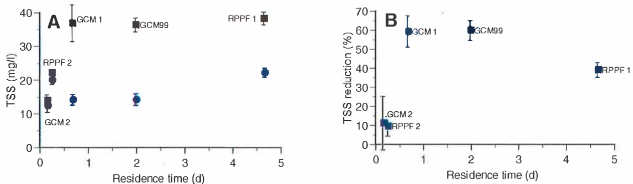
Figure 40. Change in TSS within five treatment ponds. A, input (brown squares) and discharge (blue circle) TSS concentration (mg.L -1 ). B, percent reduction in TSS (concentration difference as a proportion of initial concentration): mean \pm SE. See text and Table 2 for pond identification.
