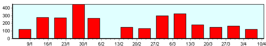
Figure 31. Total Suspended Solids (TSS) removal (kg.ha -1 .d -1 ).GCMPPF pilot treatment pond, 1999.
