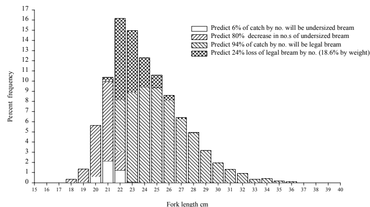
Figure 4.5. Predicted changes in the catch of undersized and legal bream when using 50 x 75 mm welded mesh back panels rather than 50 mm hexagonal mesh.
