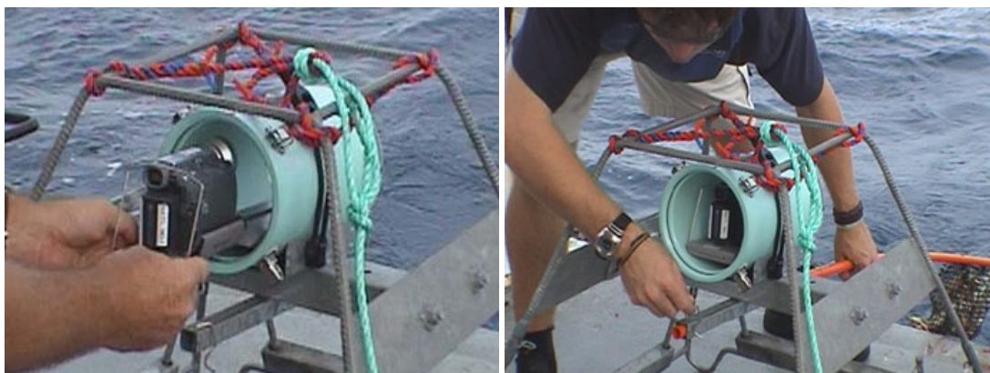
Figure 2-20: Applying camera and bait arm to BRUVS before deployment. Note ballast on frame and 8 mm hauling rope.
