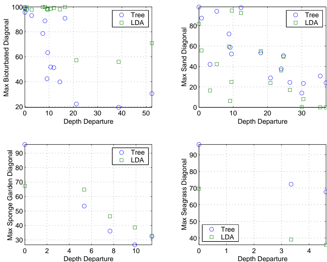
Figure 3-72: Computed four-class classification results for additional test sets, displayed as maximum confusion matrix diagonal elements for each of the four seabed classes.
