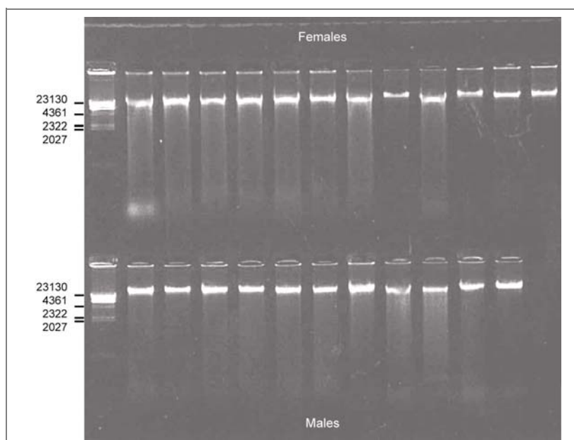
Figure 1: High quality uncut genomic DNA from 12 female and 11 male medium sized Metapenaeus macleayi which were subsequently used for telomere length assays. Molecular weight markers (bp) are shown on the left hand side.
