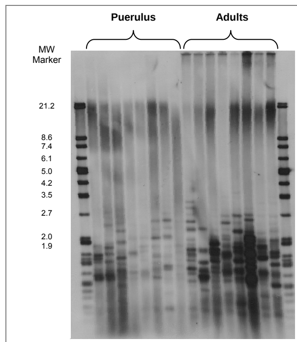
Figure 8: Autoradiograph of fluorescently-labeled telomeric restriction fragments (TRF) of young (puerulus) and older (approximately eight years old) southern rock lobster ( Jasus edwardsii ). DNA size standards are in the outer lanes.
