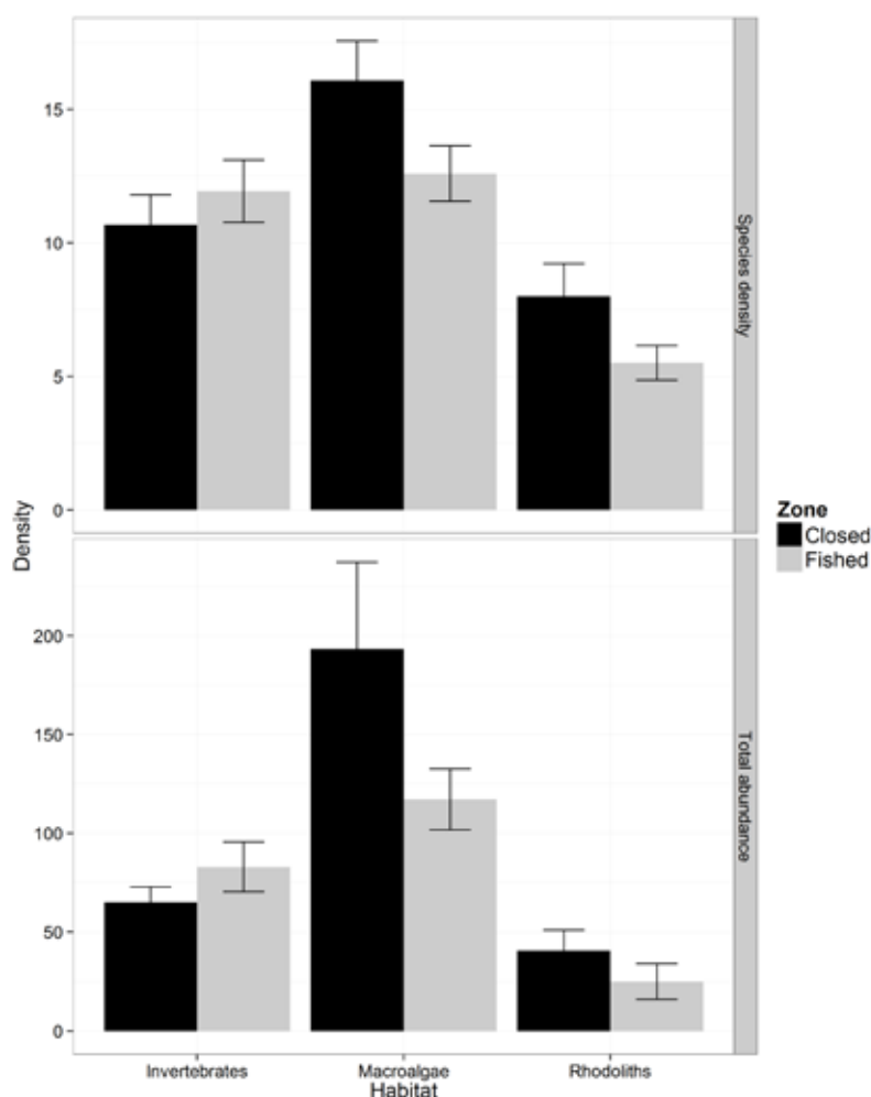
Figure 7.27. Mean species density (top) and total number of individuals (bottom) per stereo BRUV deployment for sessile invertebrates, macroalgae and rhodolith habitats between the closed (Leeman) and fished (Jurien) areas. Significant effect of habitat in the ANOVA model is indicated along with the results of pair-wise comparisons, with significant differences indicated with lower case letters
