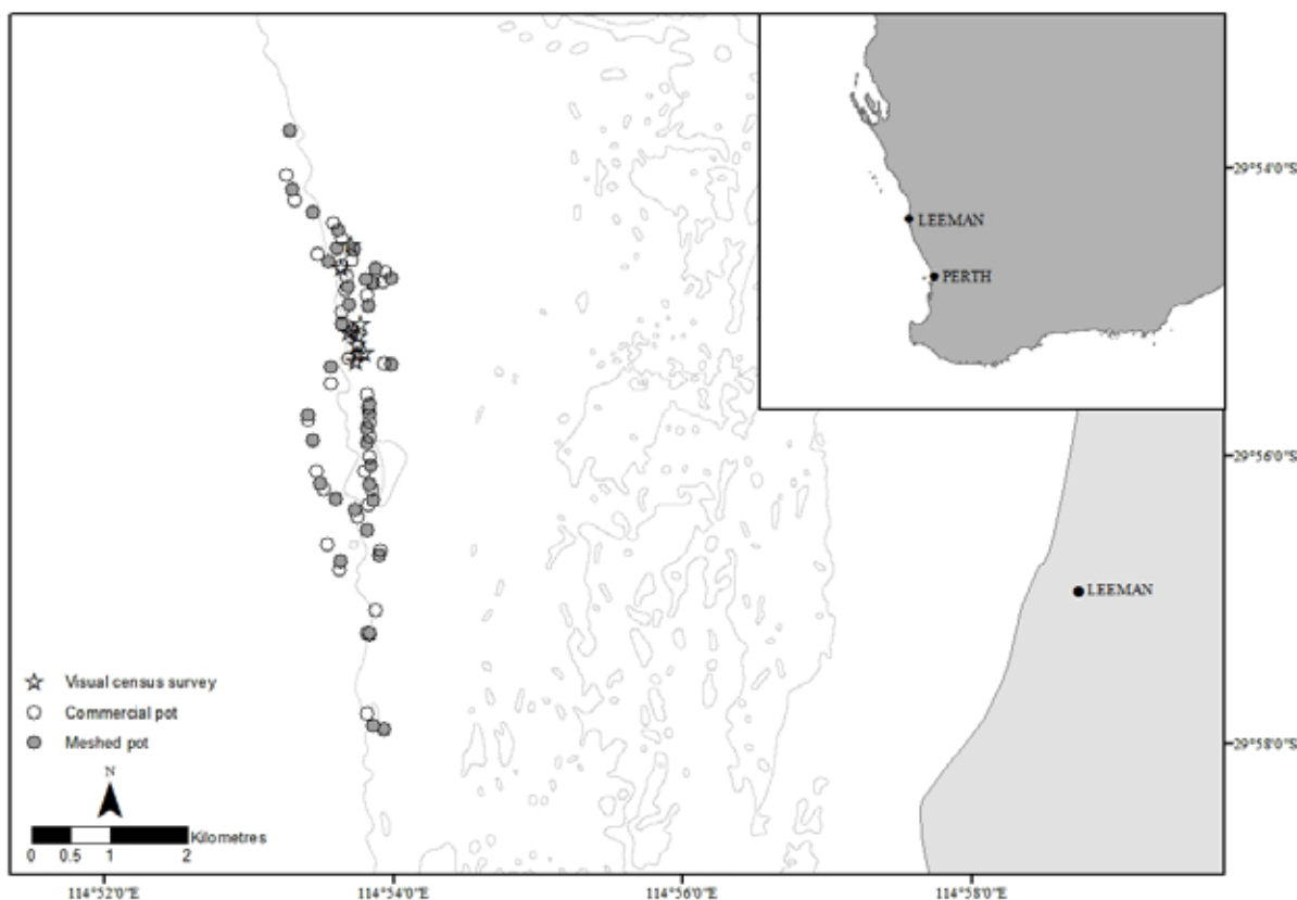
Figure 6.5. Map of medium depth (15-25m) sites west of Leeman where the sampling method comparison was conducted.
