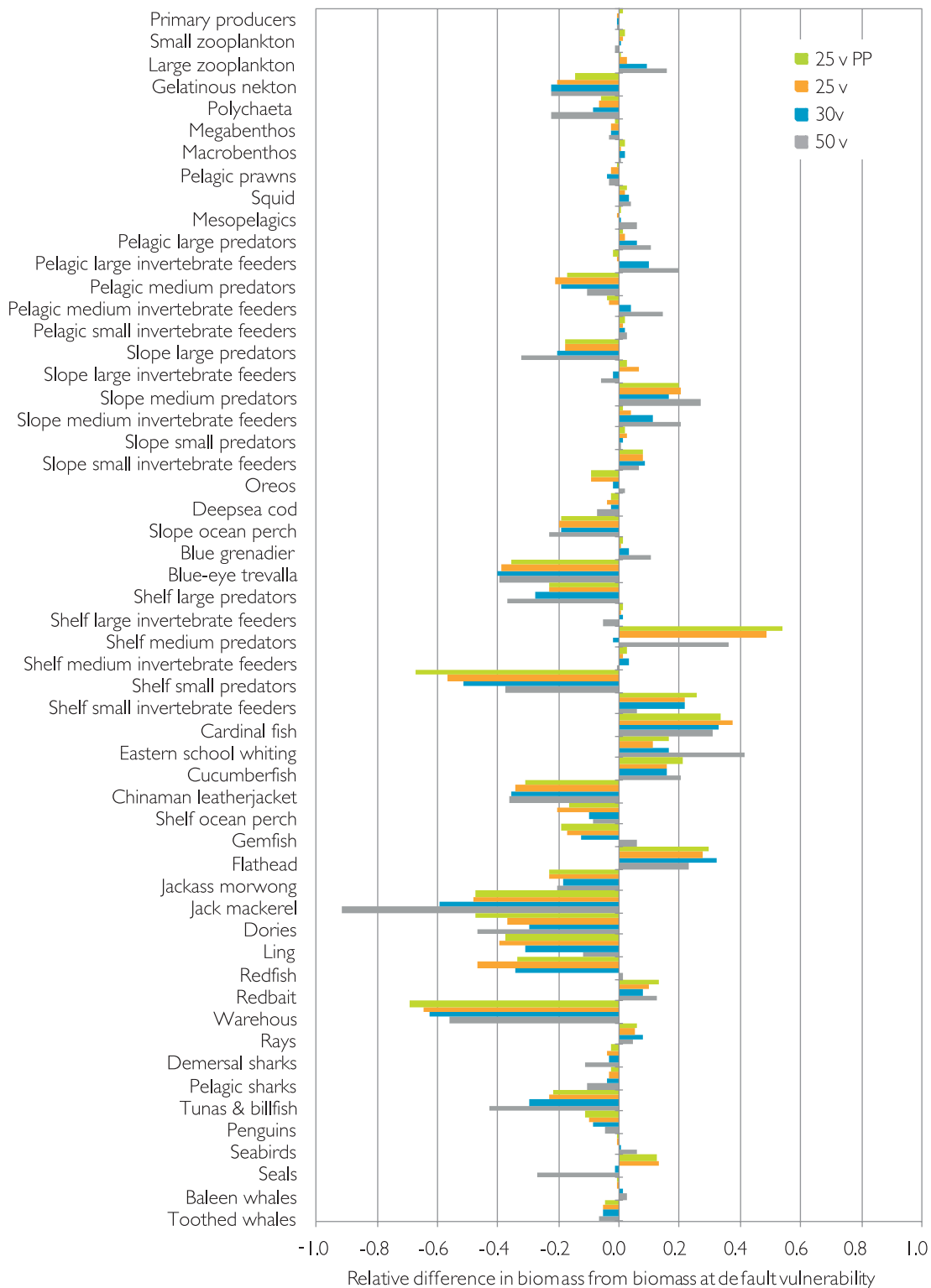
Figure 25. Relative difference in biomasses from default vulnerability biomasses for scenarios of number of fitted vulnerabilities ( n = 25, 30, 50 or 25 with the primary production forcing function also fitted) for the “red-bait fishery” EBS model.
