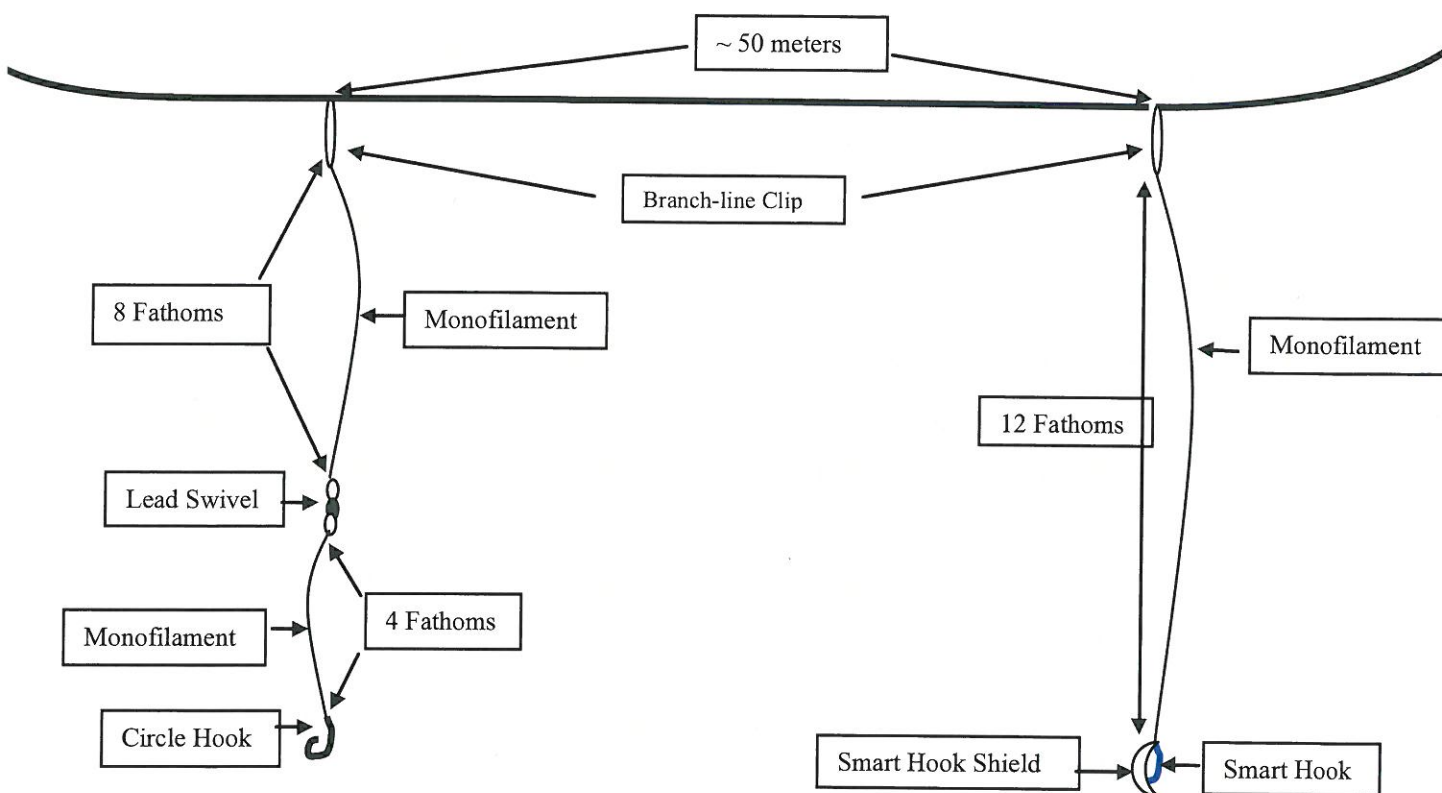
Fig 1 Gear Configuration
