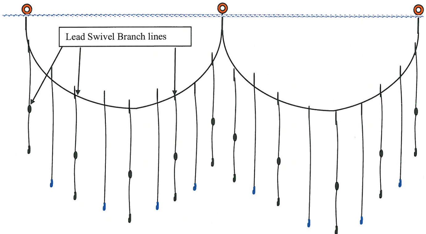
Fig 2 Mainline configuration
