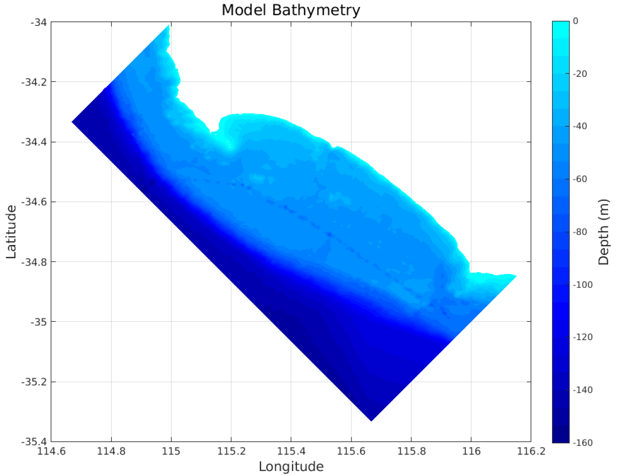
Figure 3.6 Model bathymetry
