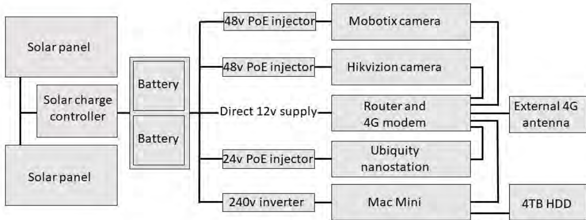
Figure 8. Schematic of camera components.
