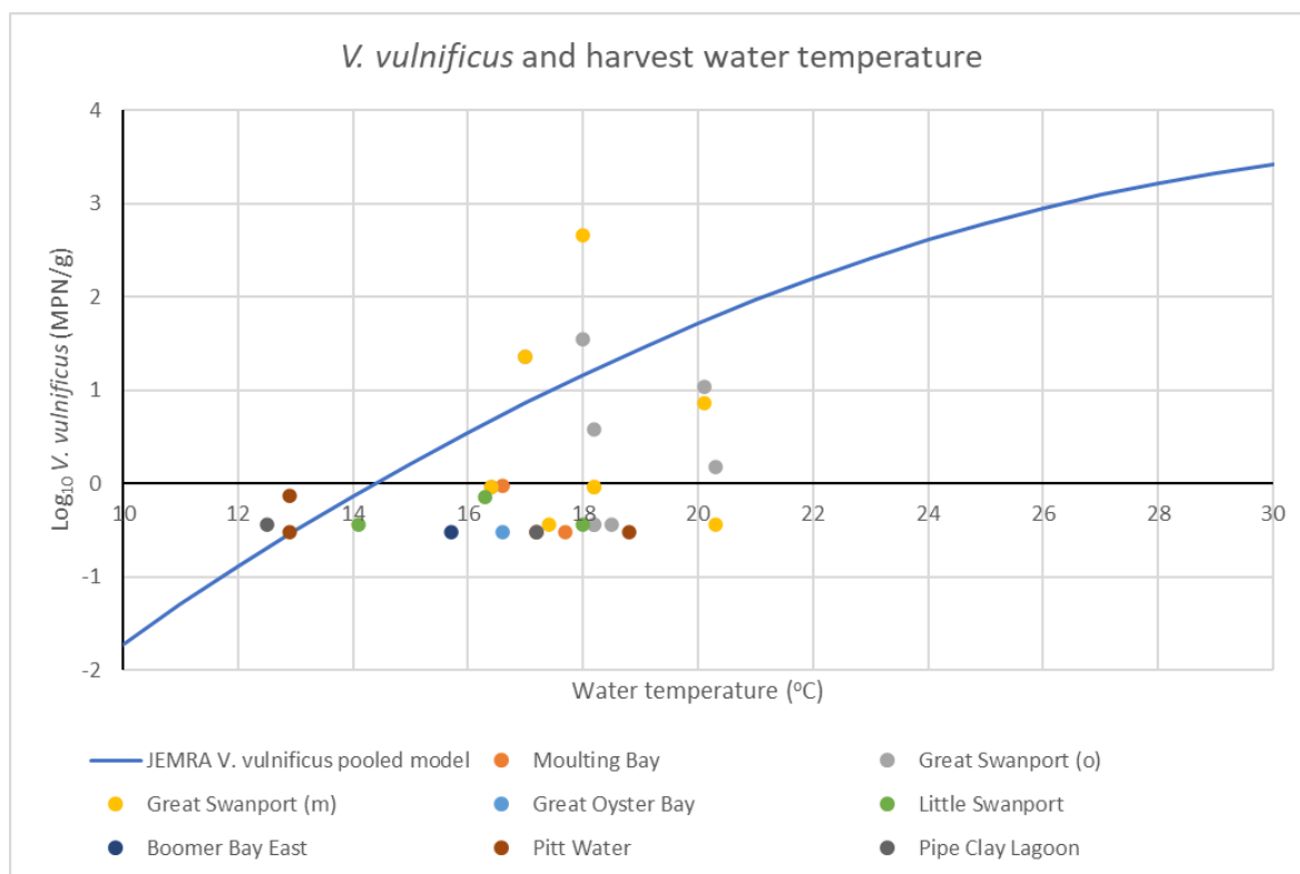
Figure 7: Vibrio vulnificus and harvest water temperature.
